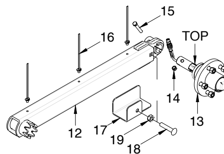
Kit S67716 Pack Control Arm - Optional
