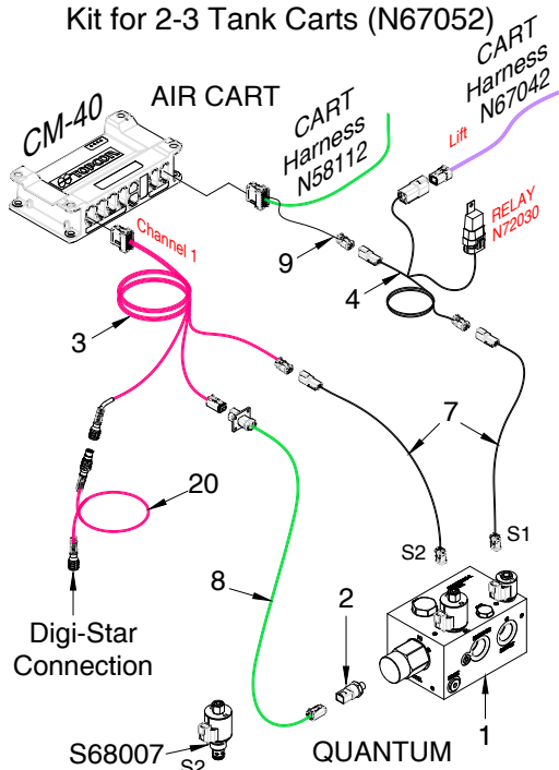
Kit for 2-3 Tank Carts (N67052)
